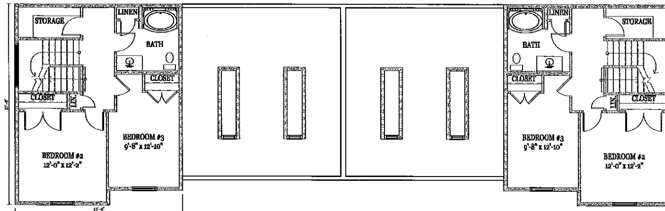
SECOND FLOOR PLAN N.T.S. 613 SQUARE FOOTAGE
