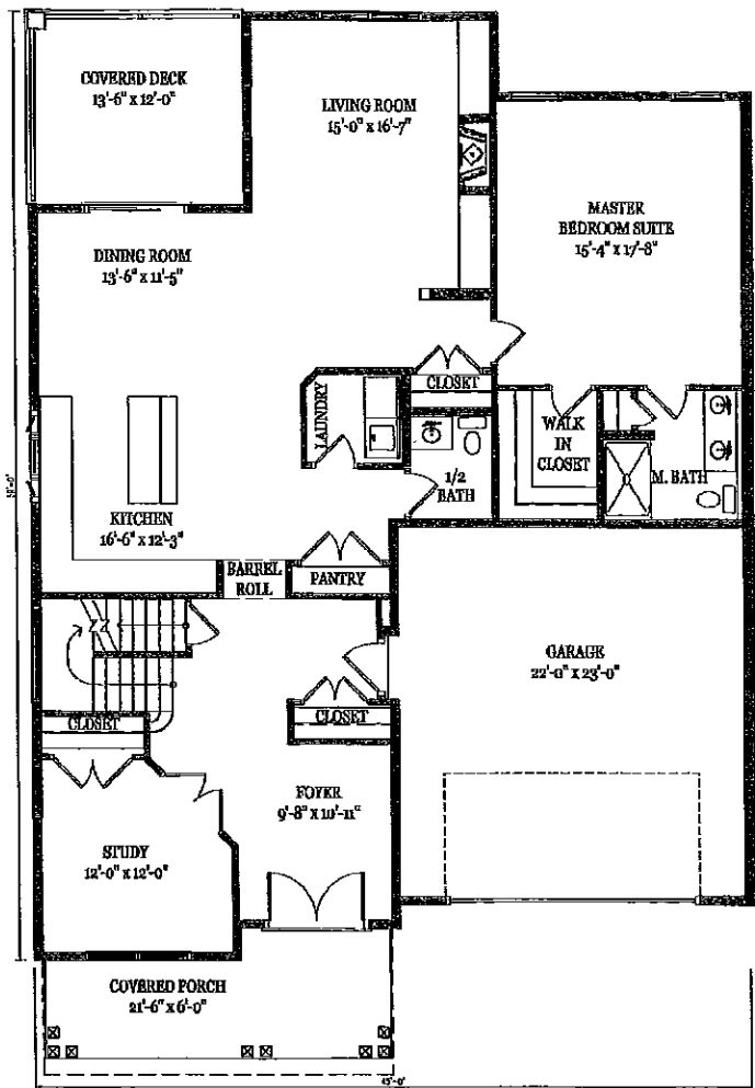
FIRST FLOOR PLAN N.T.S. 1811 SQUARE FOOTAGE
